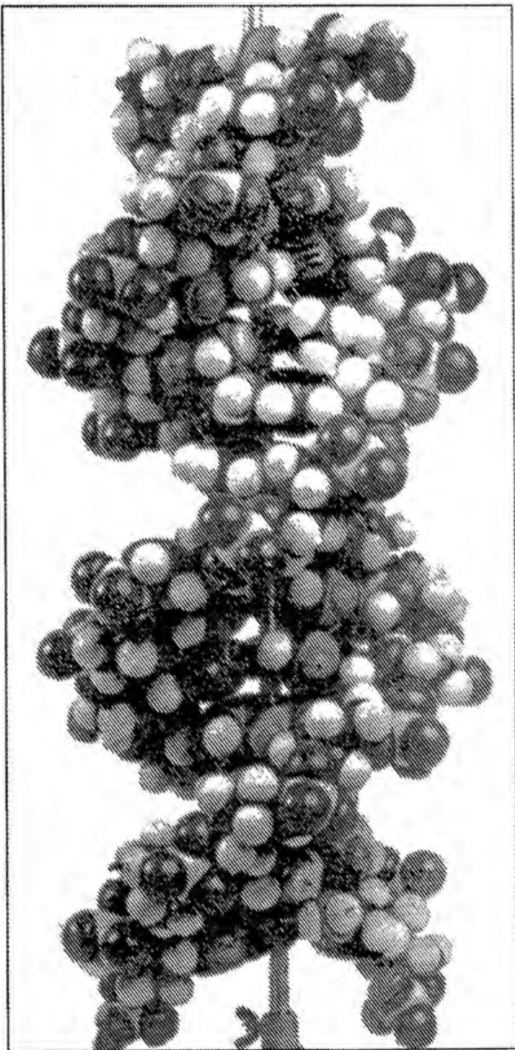
Diagram 104 DNA - Deoxyribonucleic Acid
