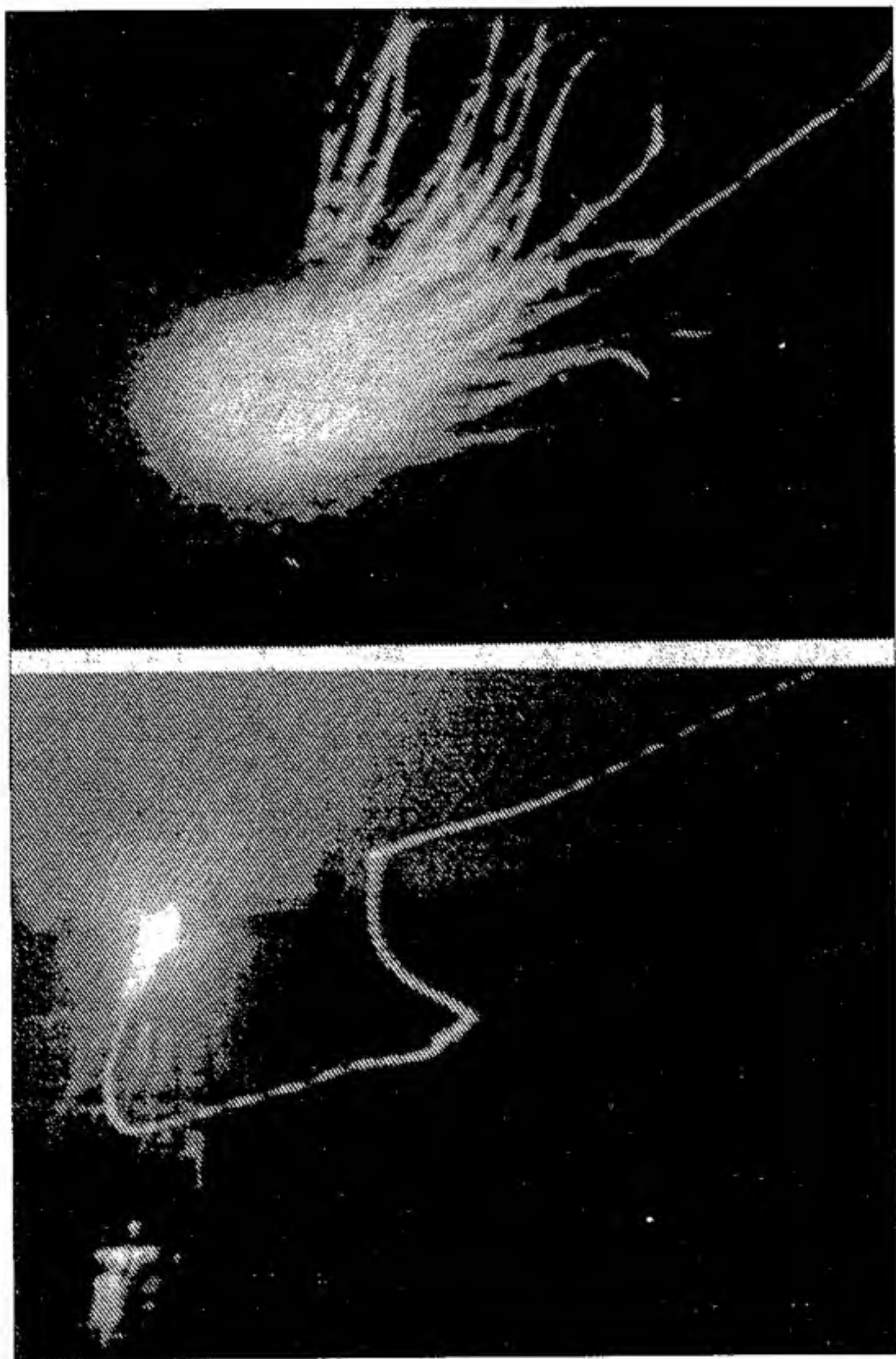
Figure 8 Ball Lightning
