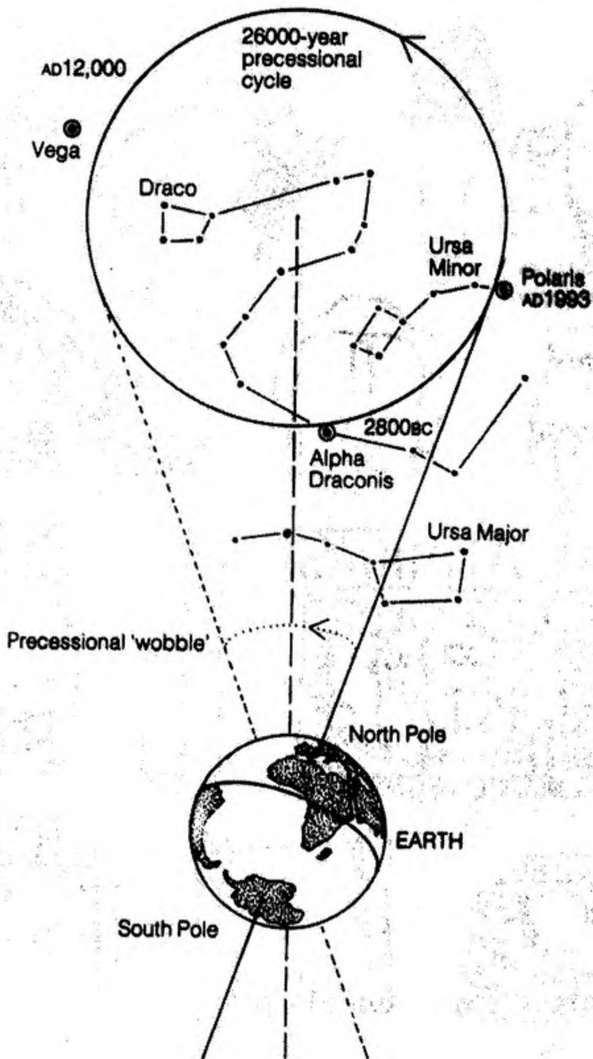
Diagram 67 Precession
