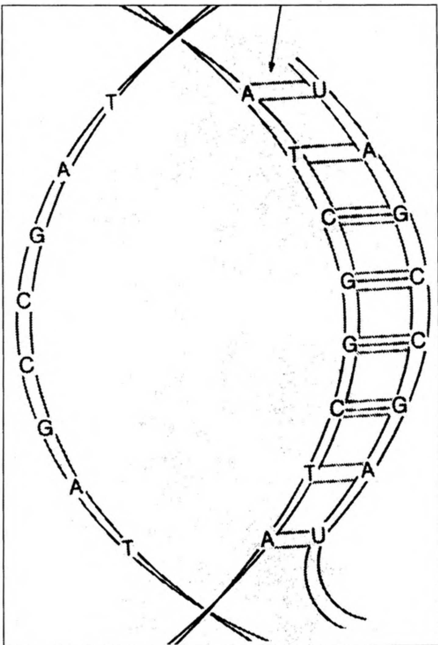
Diagram 105 RNA - Ribonucleic Acids
