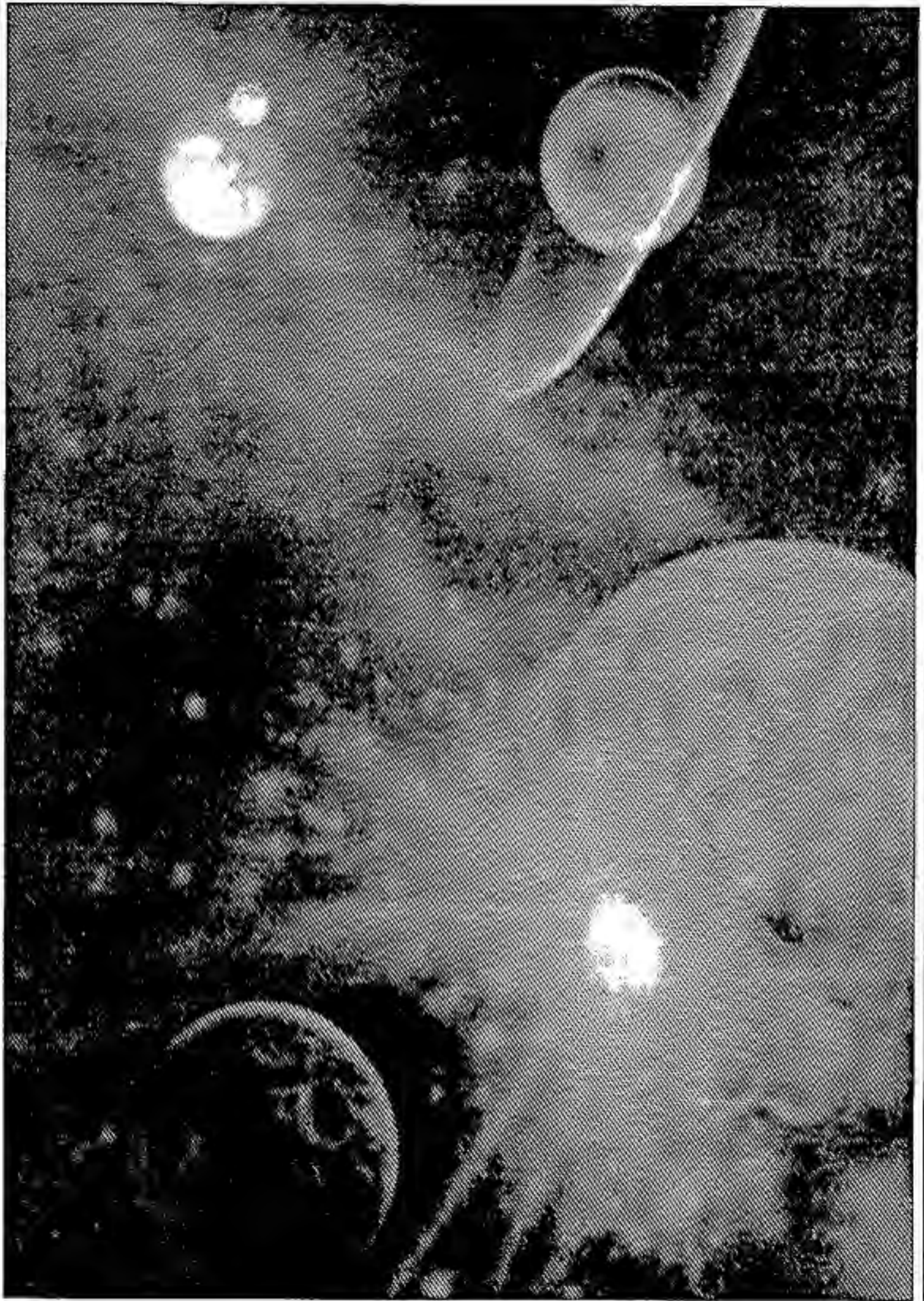
Diagram 16 The Moon Breaking Off From The Earth
